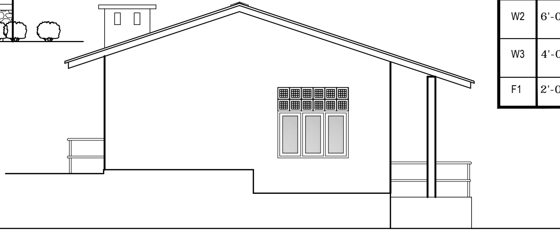
SIDE ELEVATION - P
