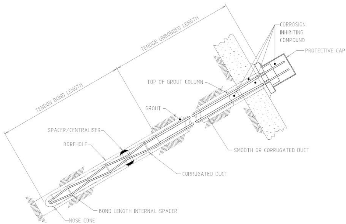
Figure 1102-3: Tendon Nomenclature
