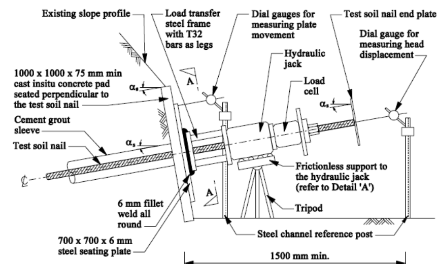
Set-up for Pullout Test
