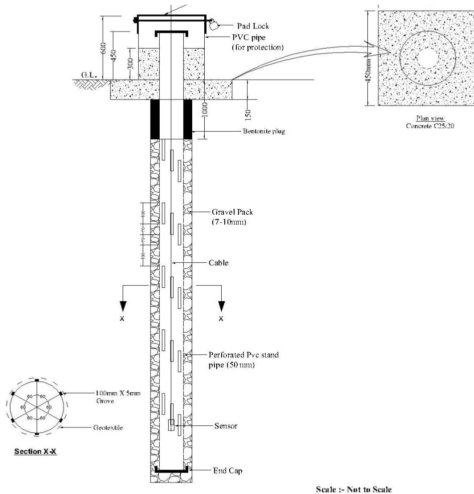
Figure 1301-4: Groundwater level gauge (Design view)
